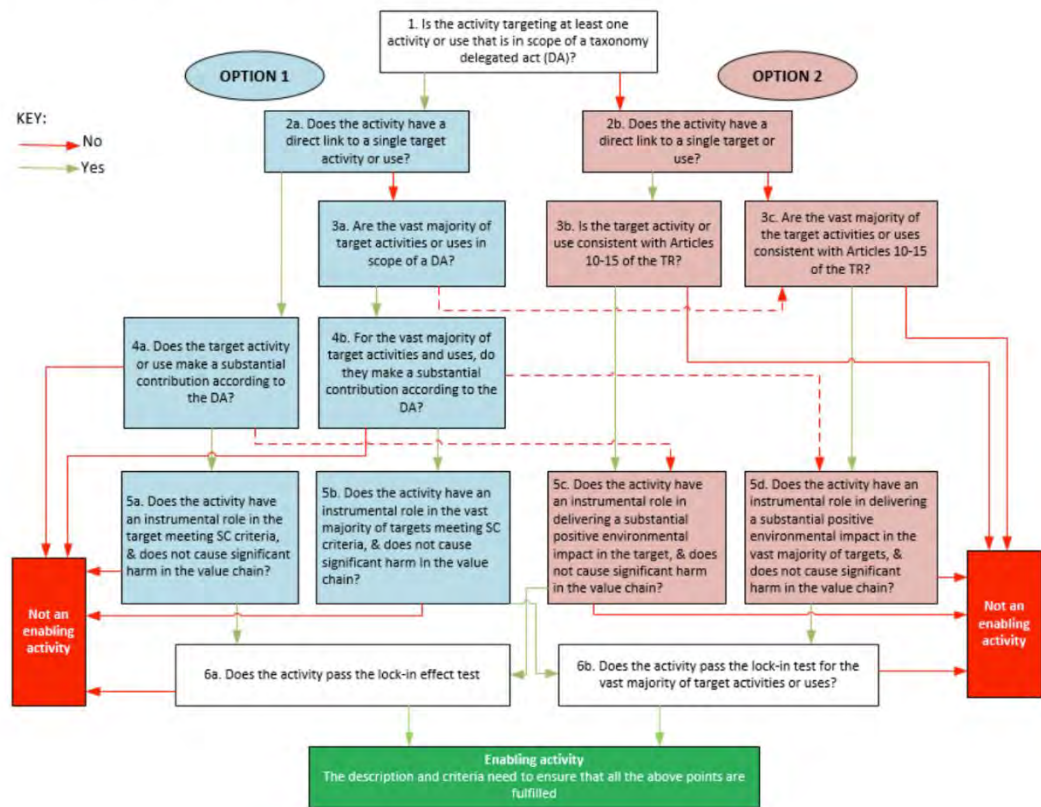
FIGURE 1: DECISION TREE
